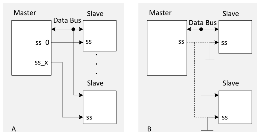
Figure 9-2 Hardware/Software Slave Selection
