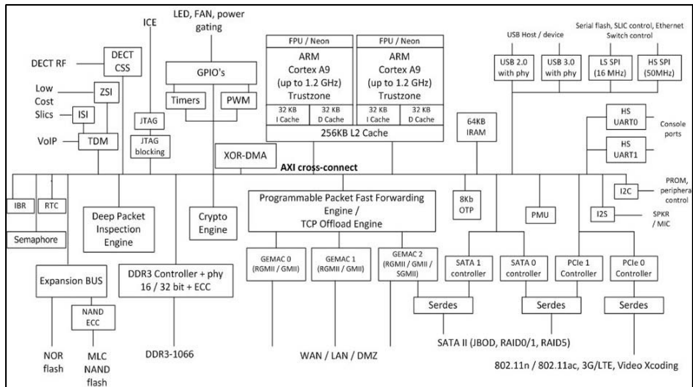
Figure 1-1 LS1024A Block Diagram
