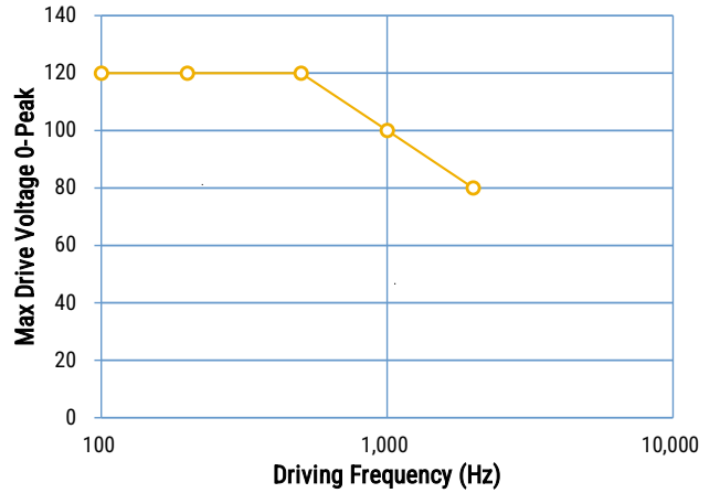
Figure 7 - Frequency vs. Max Drive Voltage Model: AS0505D20H20NF Condition: Square wave Duty 50%
