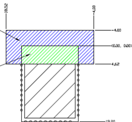
Figure 4. Recommended Host PCB Keep Out Area Around the CYBLE-0130XX-00 Antenna
