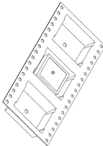
Figure 4: A5135-H tape specifications (3)
