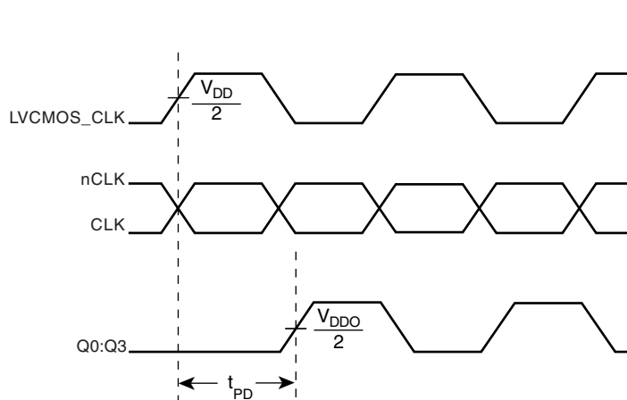
PROPAGATION DELAY
