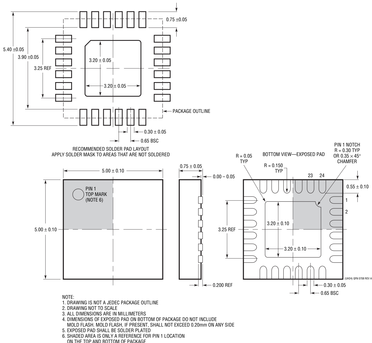
UH Package 24-Lead Plastic QFN (5mm × 5mm) (Reference LTC DWG # 05-08-1747 Rev A)
