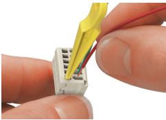
Conductor termination via operating tool (233-331) Operation parallel to conductor entry
