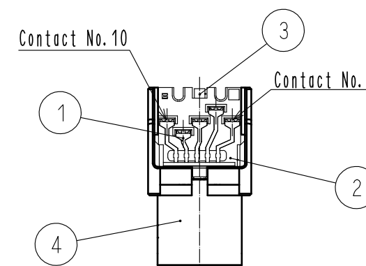
Plug Unit
