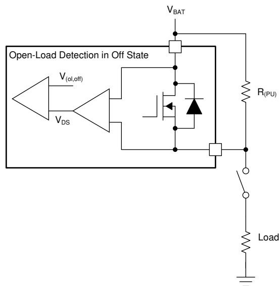
Figure 31. Open-Load Detection in Off-State
