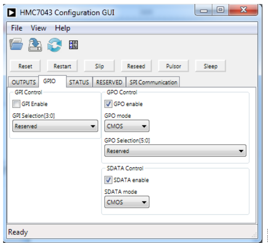
Figure 5. GPIO Tab of the HMC7043 Configuration GUI
