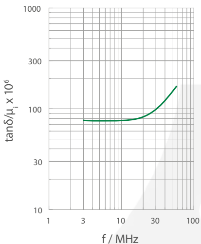
\tan\delta / \mu_i
