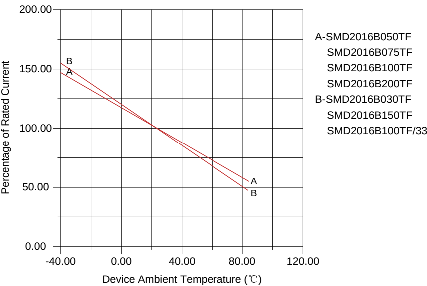
Recommended Hold Current (A) at Ambient Temperature (°C)
