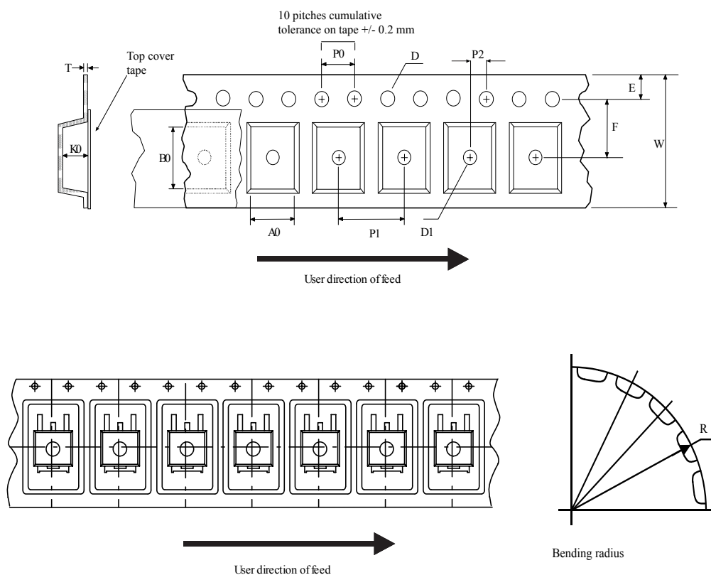
Figure 19. Tape outline
