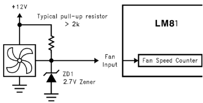
Figure 14. Fan with Tach Pull-Up to +12V and Diode Clamp
