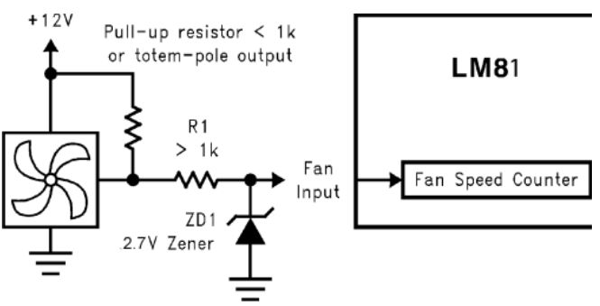
Figure 15. Fan with Strong Tach Pull-Up or Totem Pole Output and Diode Clamp
