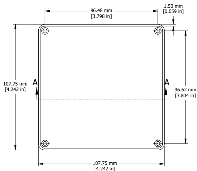
CLOSED BEZEL
