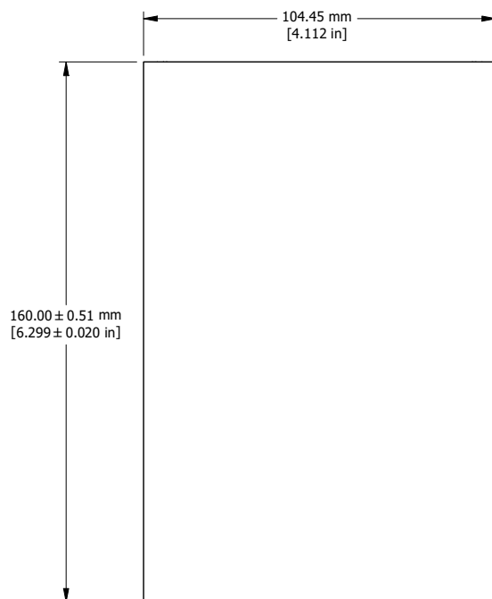
EXTRUSION
