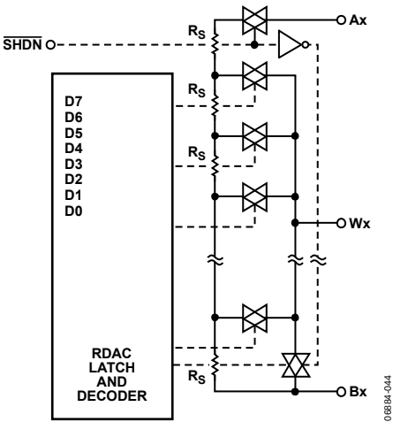
Figure 21. AD5204/AD5206 Equivalent RDAC Circuit
