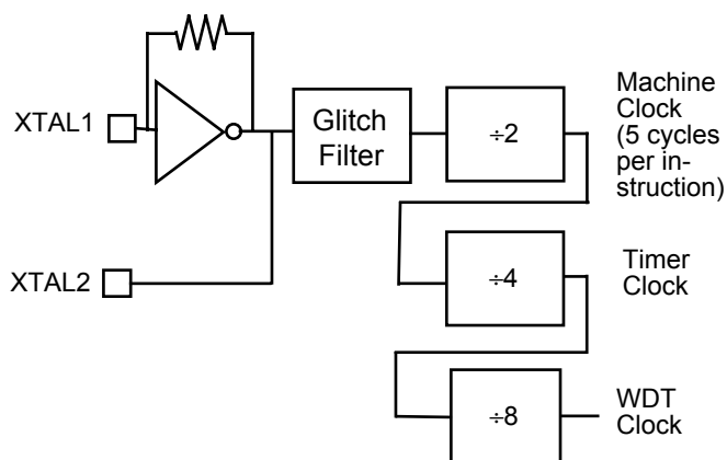
Figure 13. Z8E001 Clock Circuit
