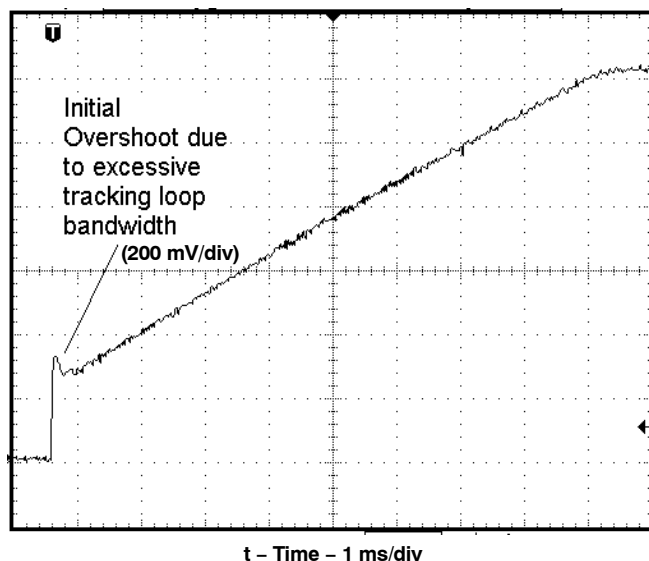
Figure 11. Excessive Tracking Loop Bandwidth
