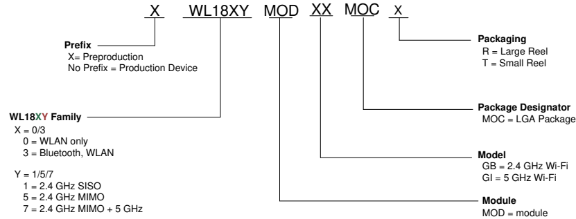
Figure 11-1. Device Nomenclature
