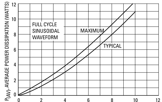
Figure 2. Power Dissipation
