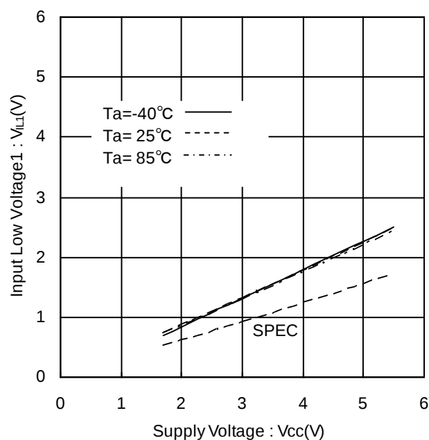
Figure 5. Input Low Voltage1 vs Supply Voltage (A0, A1, A2, SCL, SDA, WP)
