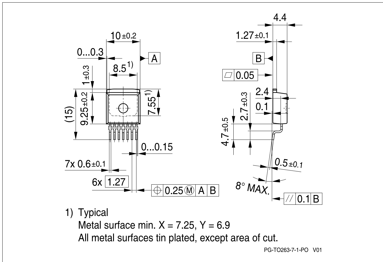
Figure 13 PG-T0263-7 1)
