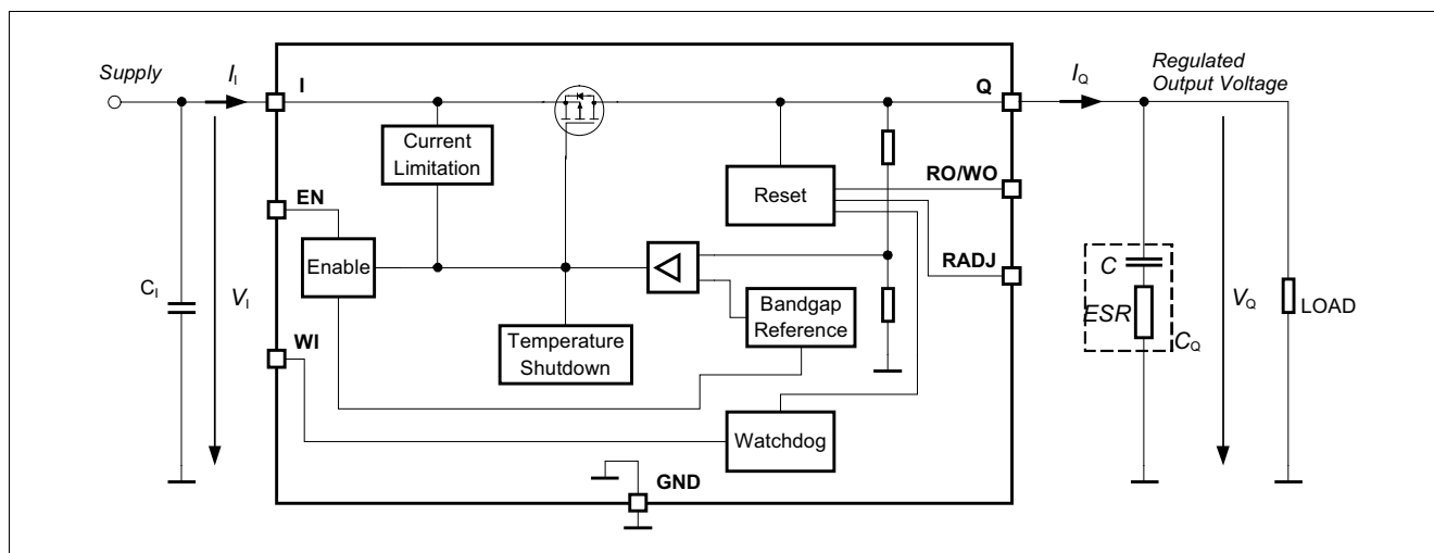
Figure 3 Voltage regulation
