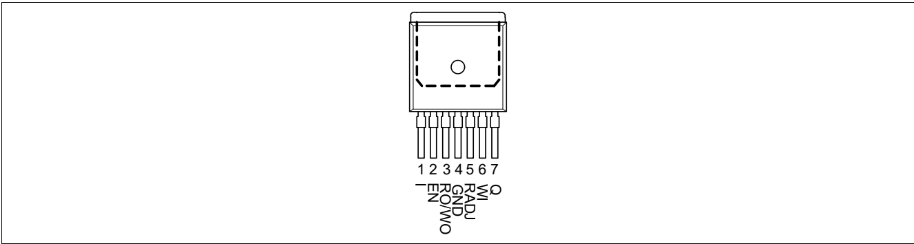
Figure 2 Pin configuration
