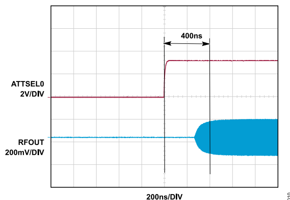
Figure 10. Gain Settling Time from Minimum Gain (AMP1/AMP2 Bypass and DSA = 24.0 dB) to Maximum Gain (No AMP Bypass and DSA = 0.0 dB)
