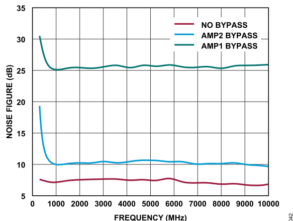
Figure 42. Noise Figure vs. Frequency for Various Bypass Modes
