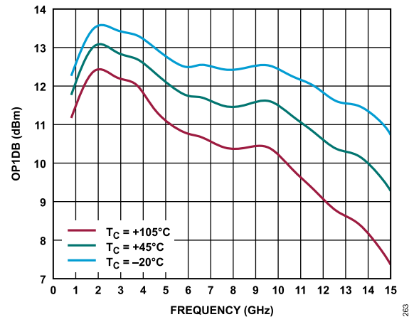
Figure 63. OP1dB vs. Frequency for Various Temperatures
