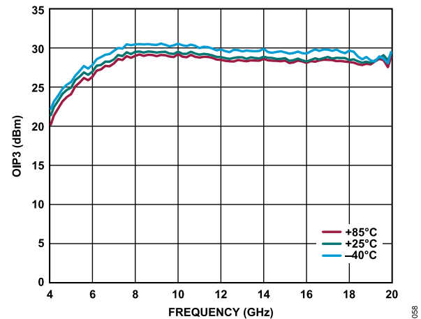
Figure 58. OIP3 vs. Frequency for Various Temperature, 4 GHz to 20 GHz, VDD = 5 V, IDQ = 90 mA, RBIAS = 7.15 kΩ
