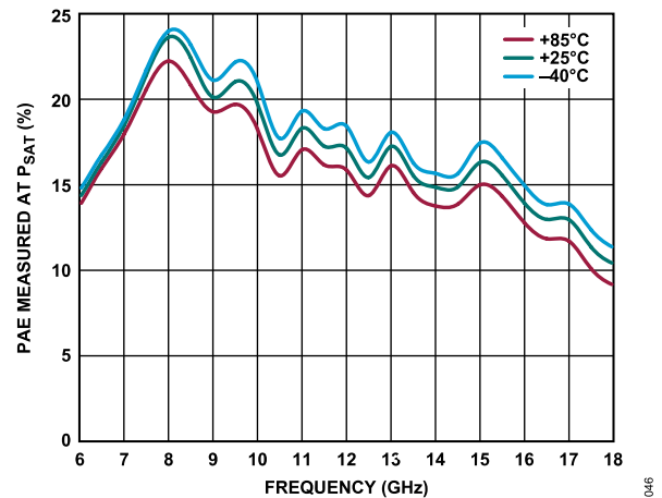
Figure 46. PAE Measured at P_{SAT} vs. Frequency for Various Temperatures, 6 GHz to 18 GHz, V_{DD} = 5\text{ V} , I_{DD} = 90\text{ mA} , R_{BIAS} = 7.15\text{ k}\Omega
