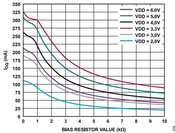
Figure 76. I_{DQ} vs. Bias Resistor Value, 1 Ω to 10 kΩ, Various Supply Voltages
