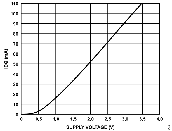
Figure 74. I_{DQ} vs. Supply Voltage, R_{BIAS} = 2.7 kΩ
