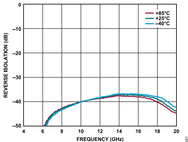
Figure 21. Reverse Isolation vs. Frequency for Various Temperatures, 4 GHz to 20 GHz, VDD = 3 V, IDQ = 90 mA, RBIAS = 2.7 kΩ
