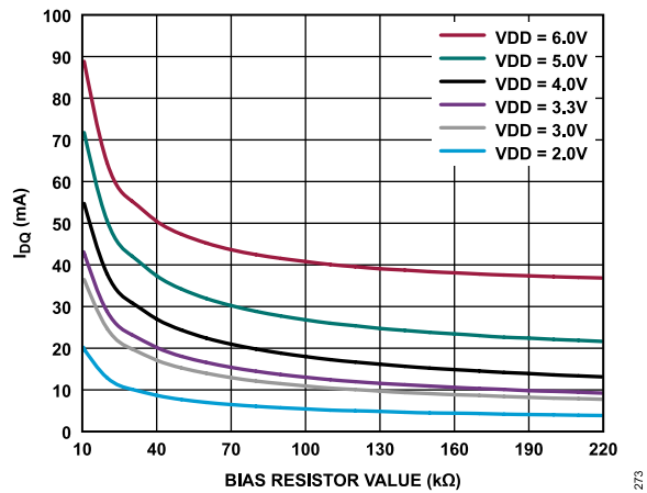
Figure 73. I_{DQ} vs. Bias Resistor Value, 10 kΩ to 220 kΩ, Various Supply Voltages
