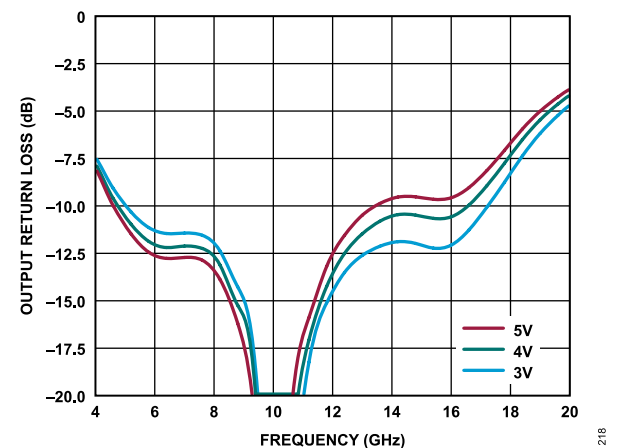
Figure 18. Output Return Loss vs. Frequency for Various Supply Voltages, I_{DQ} = 90\text{ mA}
