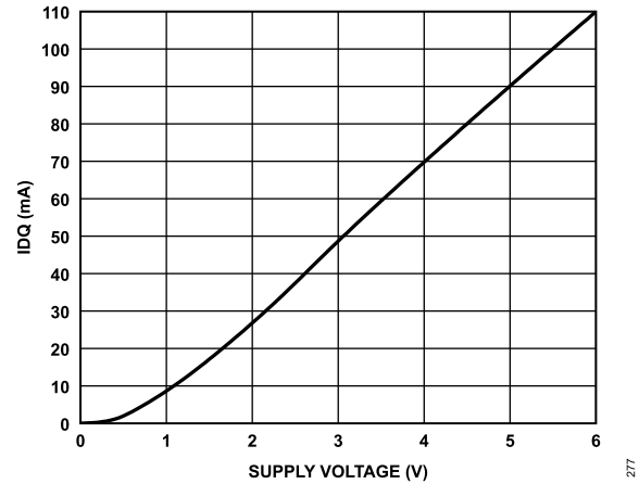
Figure 77. I_{DQ} vs. Supply Voltage, R_{BIAS} = 7.15 kΩ
