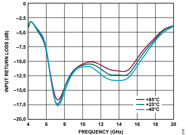
Figure 16. Input Return Loss vs. Frequency for Various Temperatures, 4 GHz to 20 GHz, V_{DD} = 5\text{ V} , I_{DQ} = 90\text{ mA} , R_{BIAS} = 7.15\text{ k}\Omega
