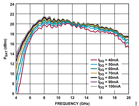
Figure 42. P_{SAT} vs. Frequency for Various I_{DQ} , VDD = 5 V
