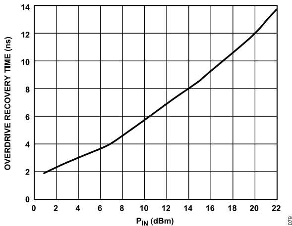
Figure 75. Overdrive Recovery Time vs. P_{IN} at 7 GHz, Recovery to Within 90% of Small Signal Gain Value, V_{DD} = 5 V, R_{BIAS} = 7.15 kΩ
