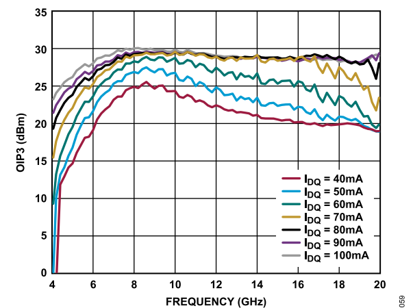
Figure 59. OIP3 vs. Frequency for Various IDQ, VDD = 5 V
