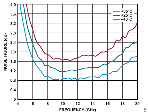
Figure 30. Noise Figure vs. Frequency for Various Temperatures, 4 GHz to 20 GHz, V_{DD} = 5 V, I_{DQ} = 90 mA, R_{BIAS} = 7.15 k \Omega
