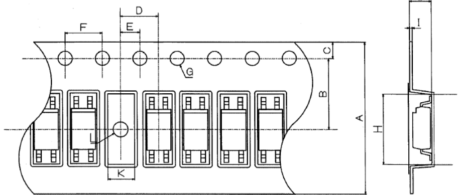
Dimensions List (Unit : mm)
