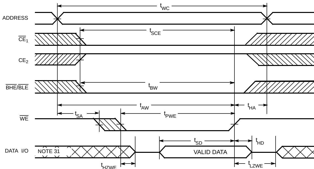
Figure 10. Write Cycle 4 ( \overline{\text{BHE/BLE}} Controlled, \overline{\text{OE}} LOW) [30, 32]
