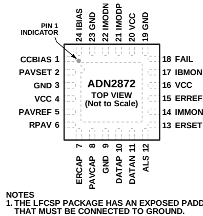
Figure 5. Pin Configuration
