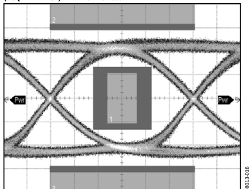
Figure 18. Optical Eye 2.488 Gbps, 65 ps/DIV, PRBS 2^{31} - 1 , PAV = -4.5 dBm, ER = 9 dB, Mask Margin 25%
