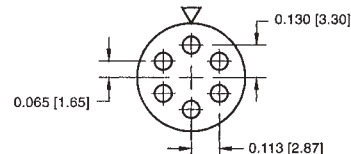
10-6 6 No. 20 Contacts
