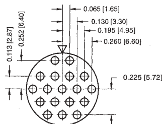
14-18 18 No. 20 Contacts
