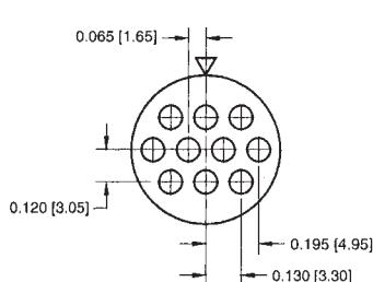
12-10 10 No. 20 Contacts
