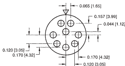
12-8 8 No. 20 Contacts
