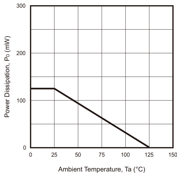
Fig.2 - Derating Curve
