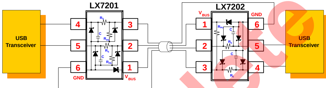
Figure 1 – Typical Application
