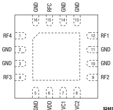
Figure 2. SKY13392-359LF Pinout – 16-Pin QFN (Top View)
