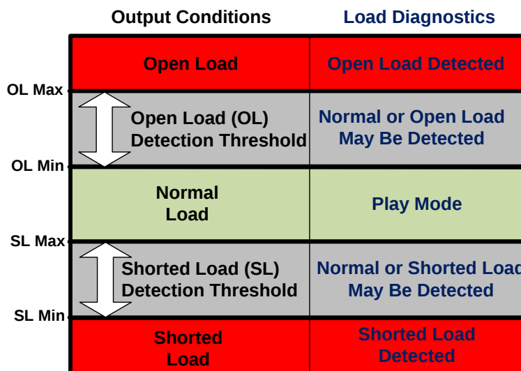
Figure 12. Load Diagnostic Reporting Thresholds
