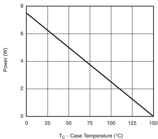
Power, Junction-to-Case
