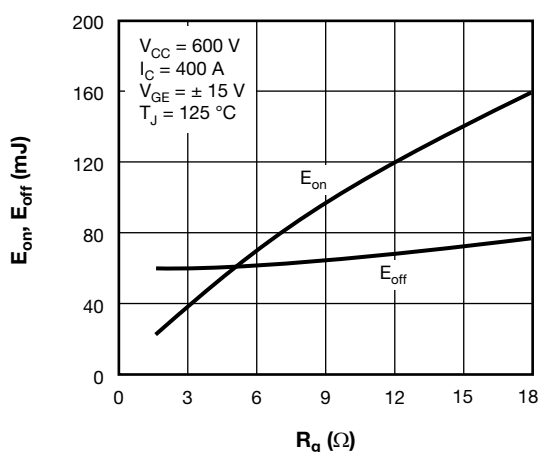
Fig. 4 - Switching Loss vs. P_g
