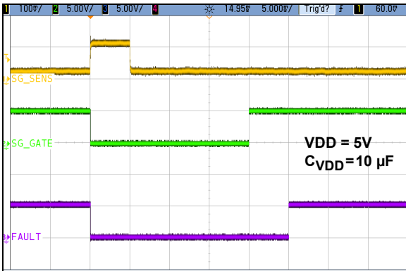
FIGURE 3-35: Battery Short-to-GND.
