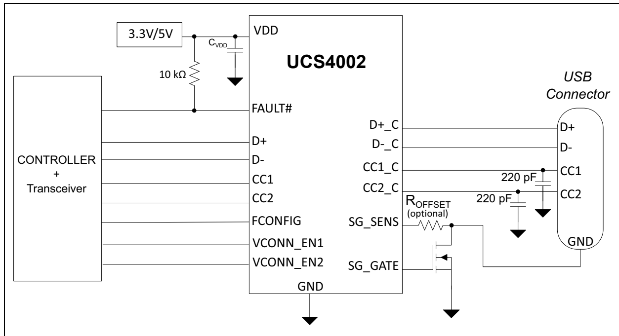
FIGURE 1-8: Typical Application.
