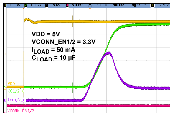
FIGURE 3-39: Hot Plug: VCONN.
