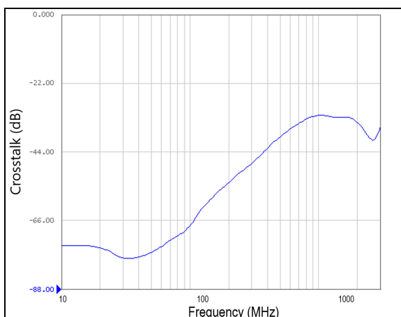
FIGURE 3-14: D+/- Crosstalk.
