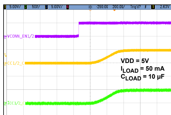
FIGURE 3-40: Turn ON with VCONN_EN1/2: VCONN.
