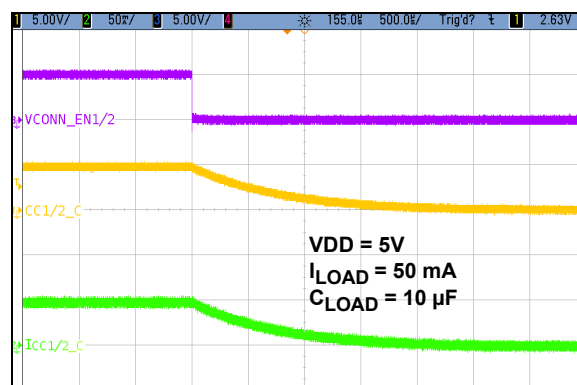
FIGURE 3-41: Turn OFF with VCONN_EN1/2: VCONN.
