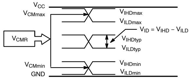
Figure 8. V_{CM} Diagram
