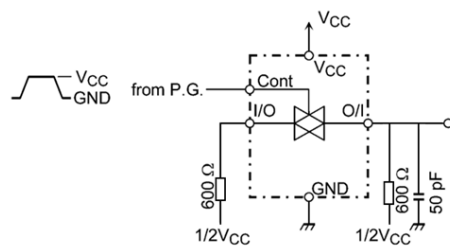
Figure 4 Feedthrough Attenuation
