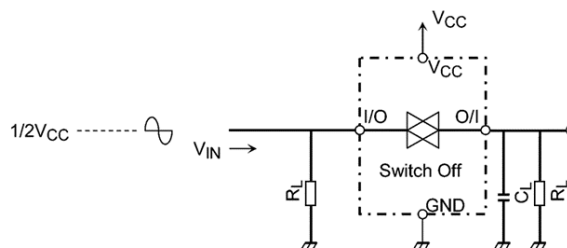
Figure 4 Feedthrough Attenuation
