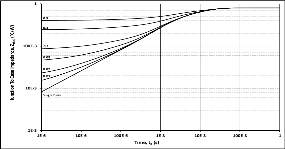
Figure 9 Transient Thermal Impedance
