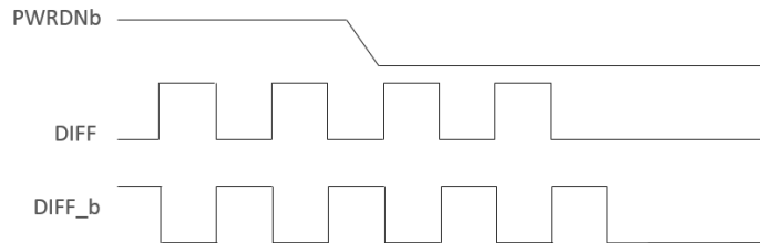
Figure 13. PWRDNb Assertion
