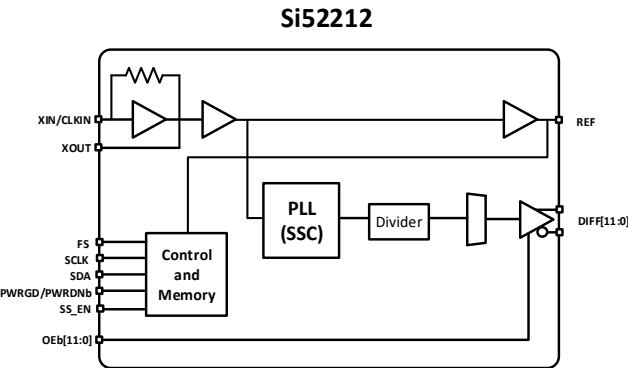
Figure 1. Si52212 Block Diagram 12-Output, 64-QFN
