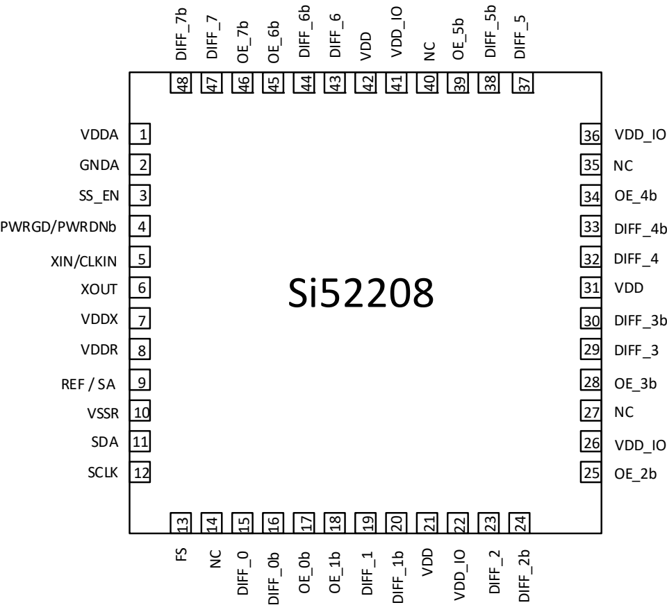
Figure 6. Si52208 48-pin QFN Pinout
