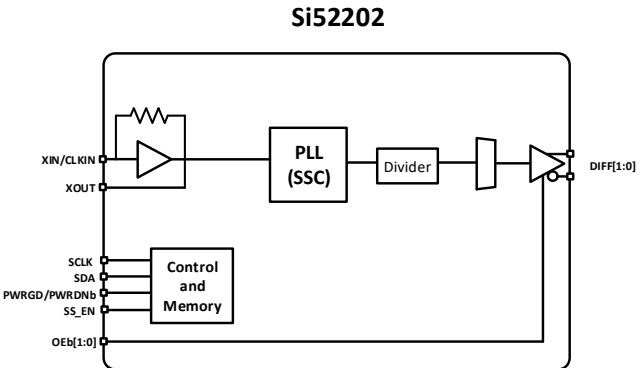
Figure 4. Si52202 Block Diagram 2-Output, 20-QFN
