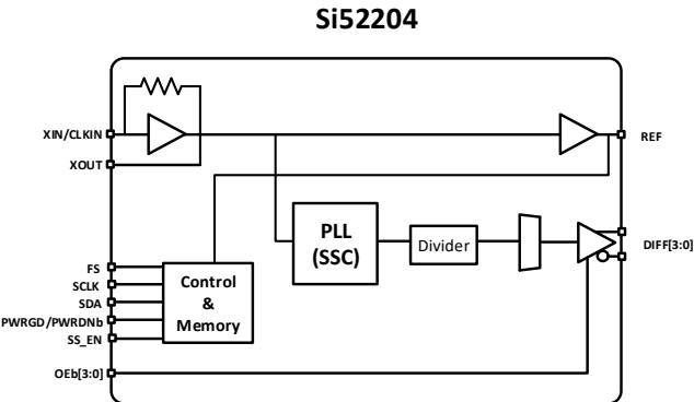
Figure 3. Si52204 Block Diagram 4-Output, 32-QFN
