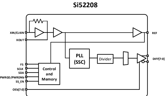
Figure 2. Si52208 Block Diagram 8-Output, 48-QFN
