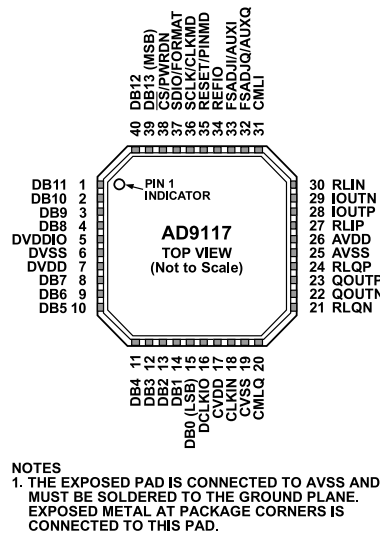
Figure 5. AD9117 Pin Configuration
