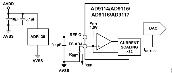
Figure 97. External Reference Configuration
