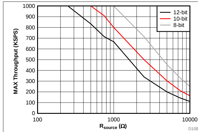
Figure 64. 2xV_{REF} Input Range Settling Without an MXO Buffer
