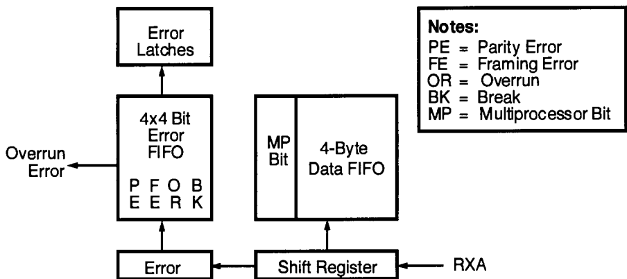
Figure 22. ASCI Receiver
