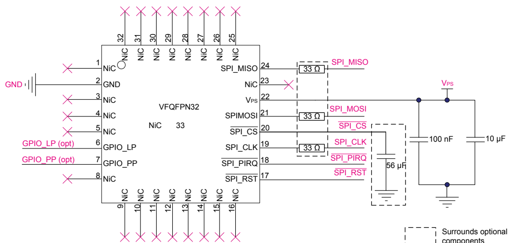
Figure 11. Typical hardware implementation (VFQFPN32 package)
