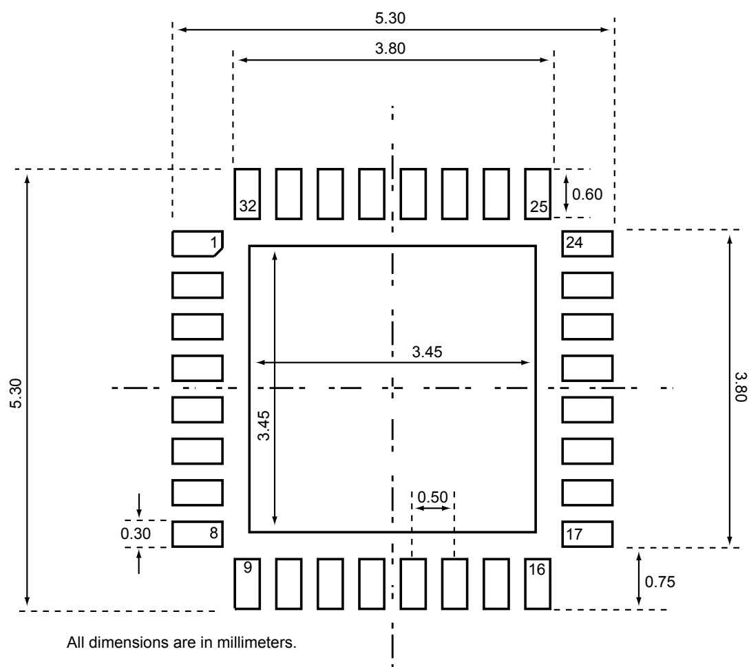
Figure 14. VFQFPN32 - recommended footprint
