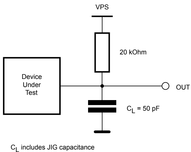
Figure 10. AC testing load circuit
