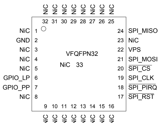
Figure 1. VQFN32 pinout
