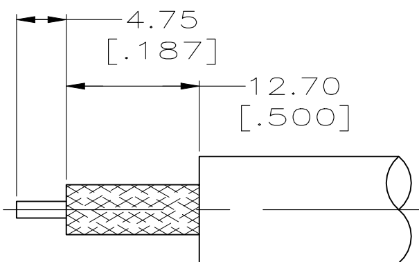
RECOMMENDED STRIP LENGTH NO SCALE FOR 5225554-9 AND 1-5225554-1
