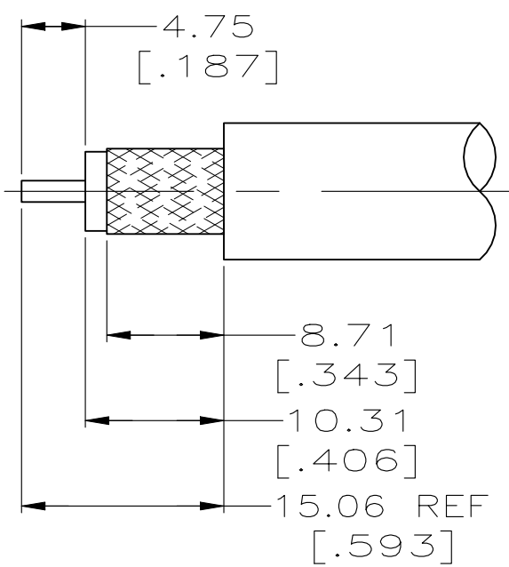
RECOMMENDED STRIP LENGTH NO SCALE FOR 5225554-2 AND 5225554-6
