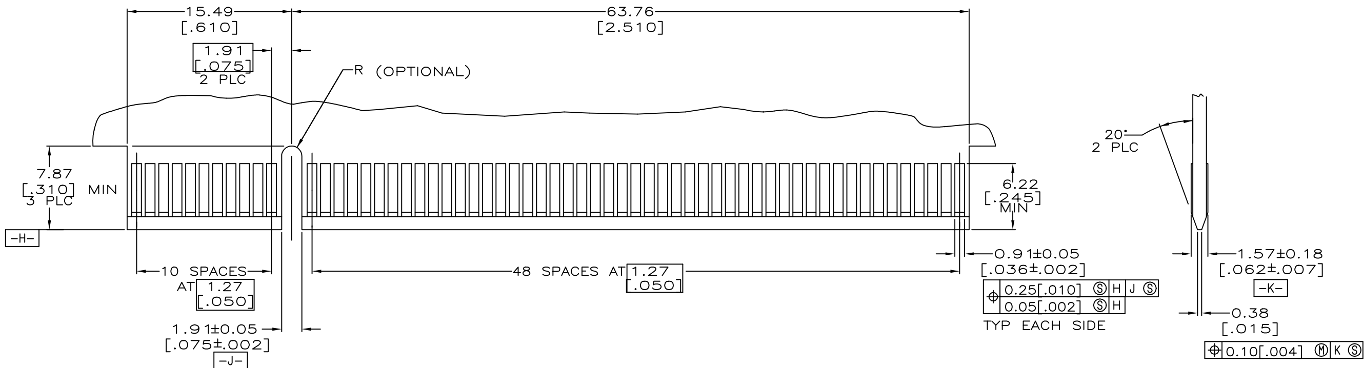
RECOMMENDED MATING BOARD EDGE CONFIGURATION
