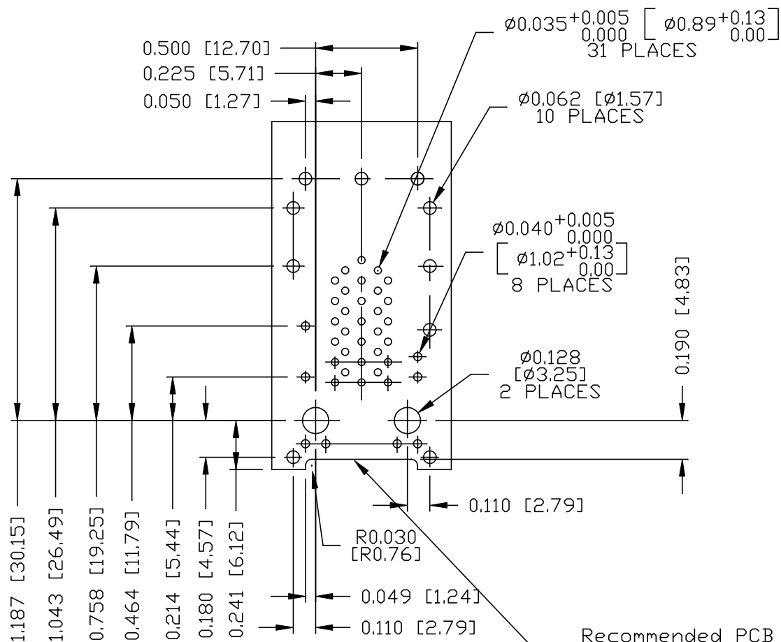
SUGGESTED FOOTPRINT (COMPONENT SIDE VIEW)
