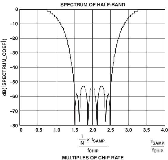
Figure 32. Interpolating Half-Band Frequency Response
