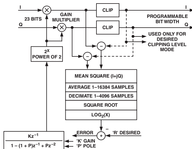
Figure 33. Block Diagram of the AGC
