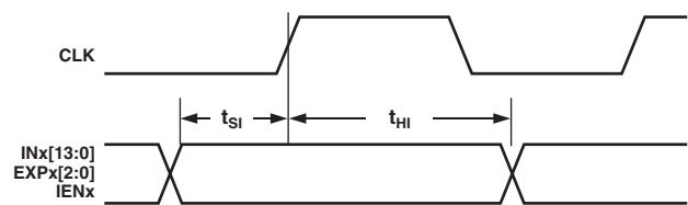
Figure 6. Input Timing for A and B Channels
