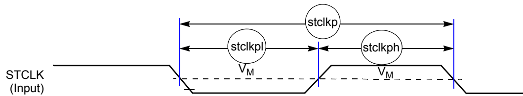
Figure 80. STCLK Timing
