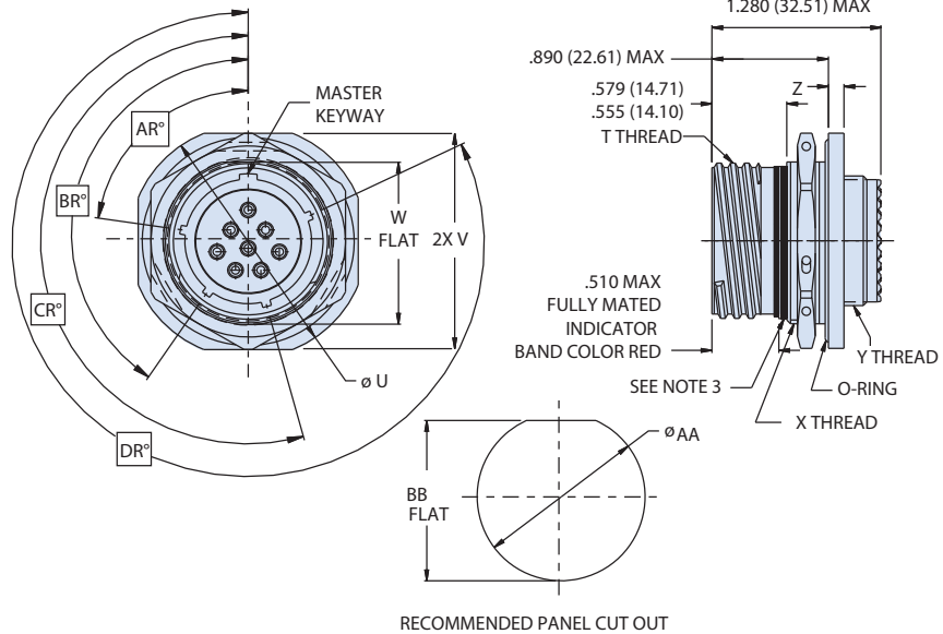
RECOMMENDED PANEL CUT OUT
