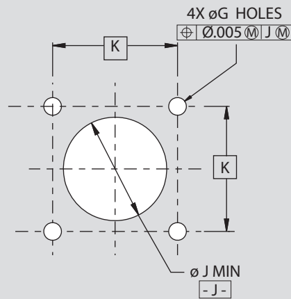
Wall or Box Mount Front Panel Mounting
