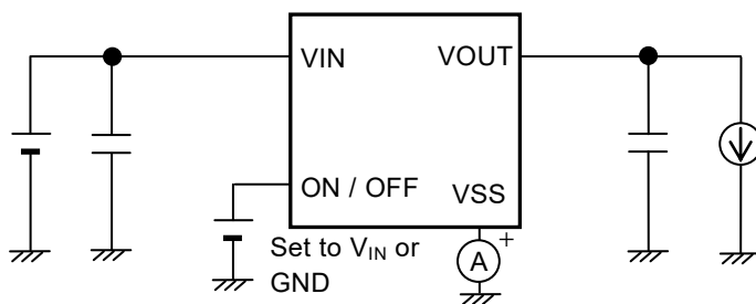
Figure 6 Test Circuit 2
