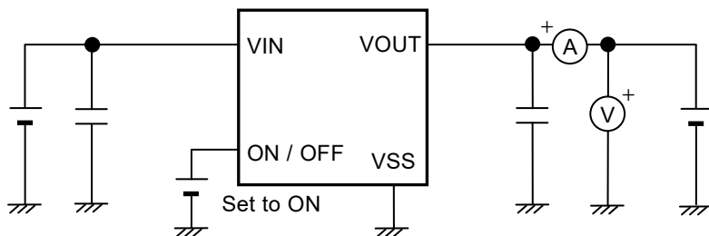
Figure 7 Test Circuit 3
